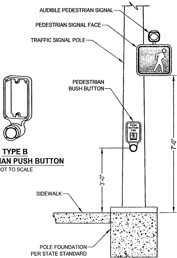
COMBINED TRAFFIC SIGNAL PEDESTRIAN PUSH BUTTON POLE NOT TO SCALE
