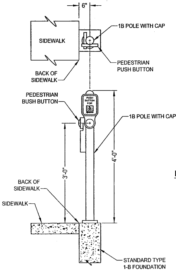
PEDESTRIAN PUSH BUTTON POLE NOT TO SCALE
